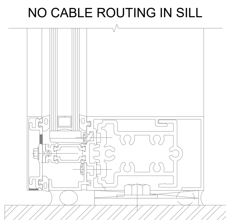
DETAIL 3 SILL
