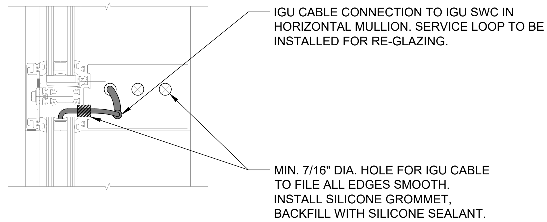
DETAIL 2 HORIZONTAL MULLION
